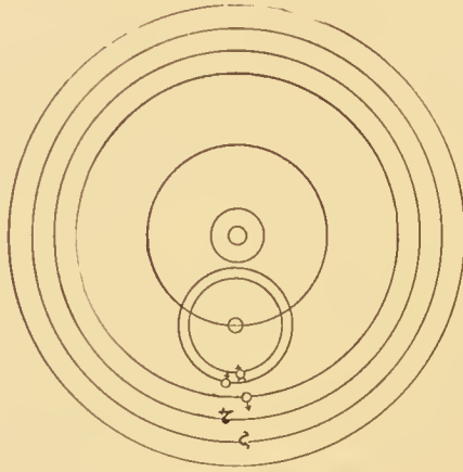
FIG. 11.—Egyptian system.
